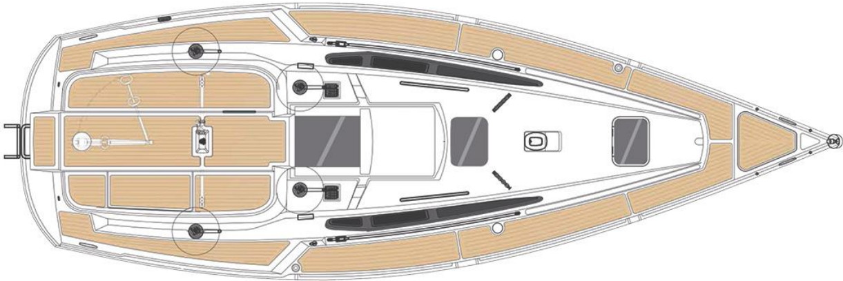
DECK LAYOUT
